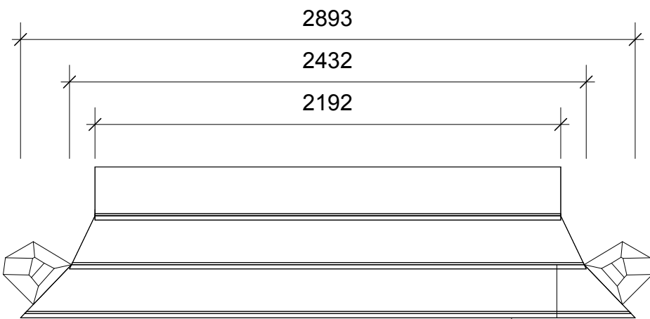
01 Staircase Piece 1 Top Scale 1:25
