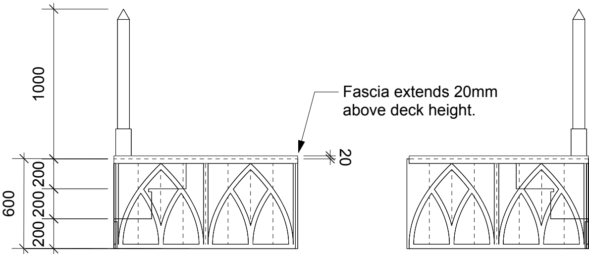
01 Chapel Stage Front Scale 1:25
