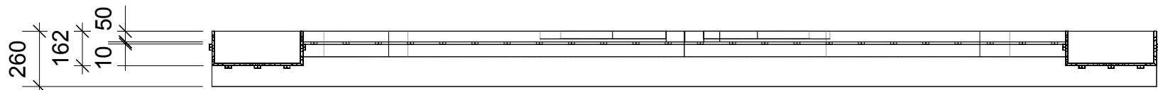
02 Chapel Wall Top Scale 1:25
