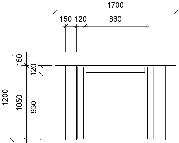
01 Fireplace Front Scale 1:25
