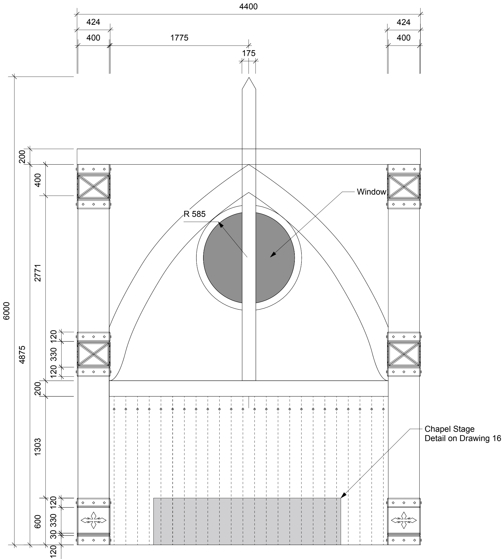
01 Chapel Wall Front Scale 1:25
