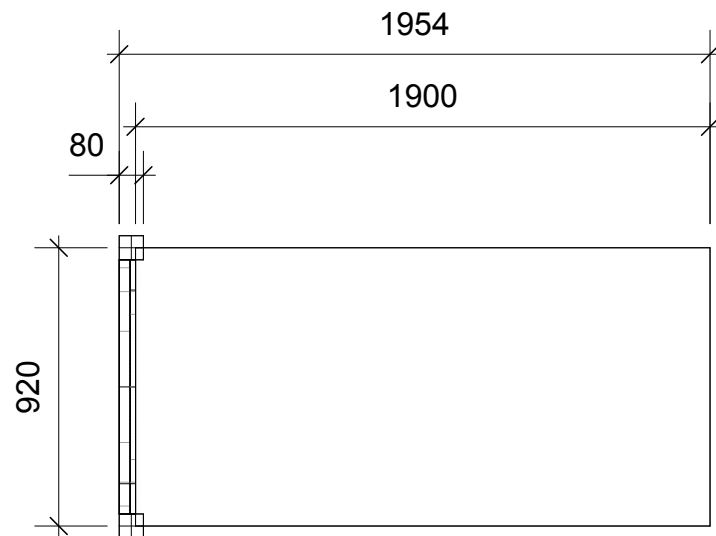
01 Bed Front Scale 1:25
