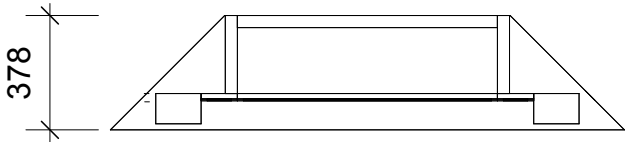
02 Fireplace Top Scale 1:25
