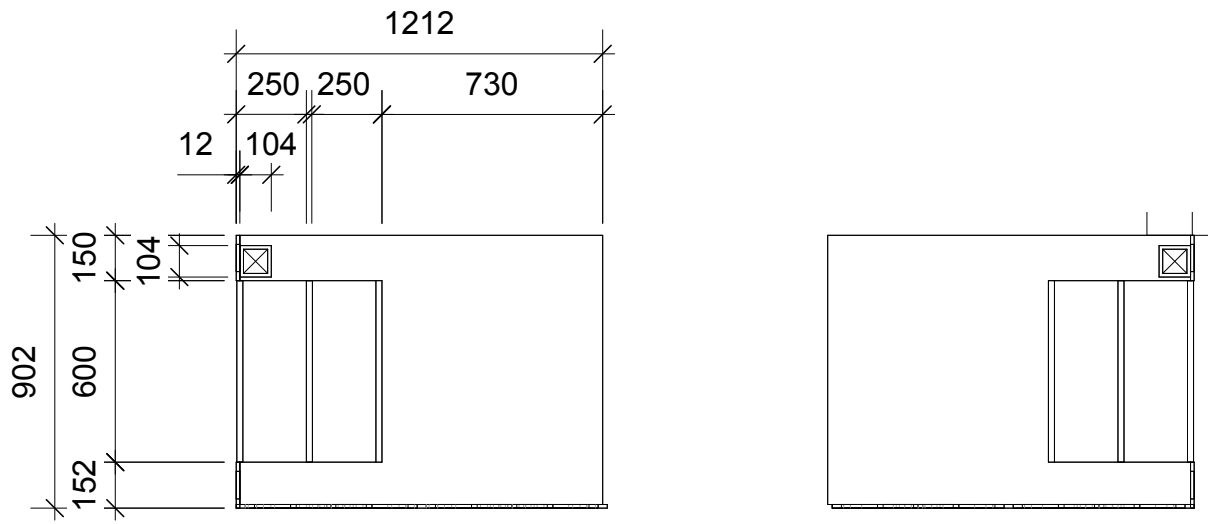
02 Chapel Stage Top Scale 1:25
