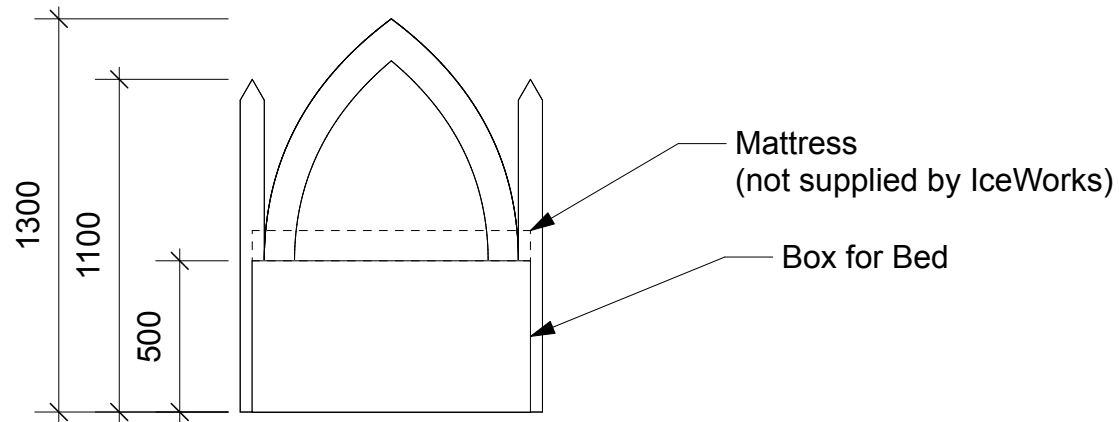
02 Bed Side Scale 1:25
