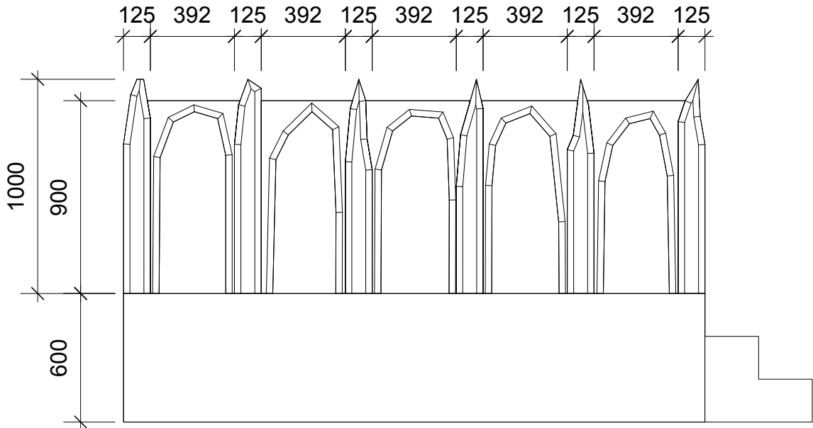
02 Staircase Piece 2 Front Scale 1:25
