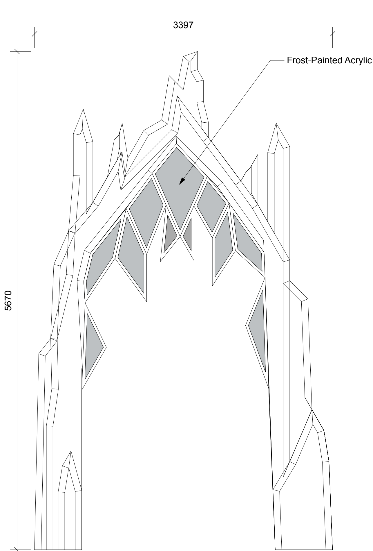
04 Ice Palace Front Scale 1:25
