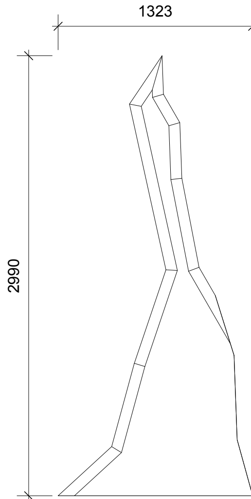
07 Ice Palace PS Layer 2 Scale 1:25
