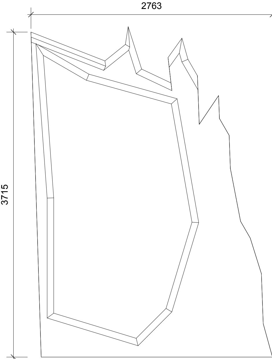
06 Ice Palace PS Layer 1 Scale 1:25
