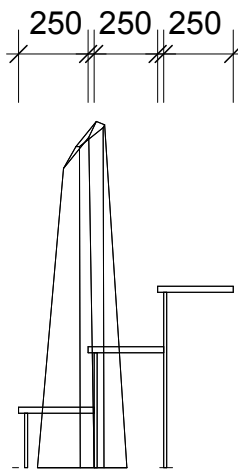
03 Staircase Piece 1 Side Scale 1:25
