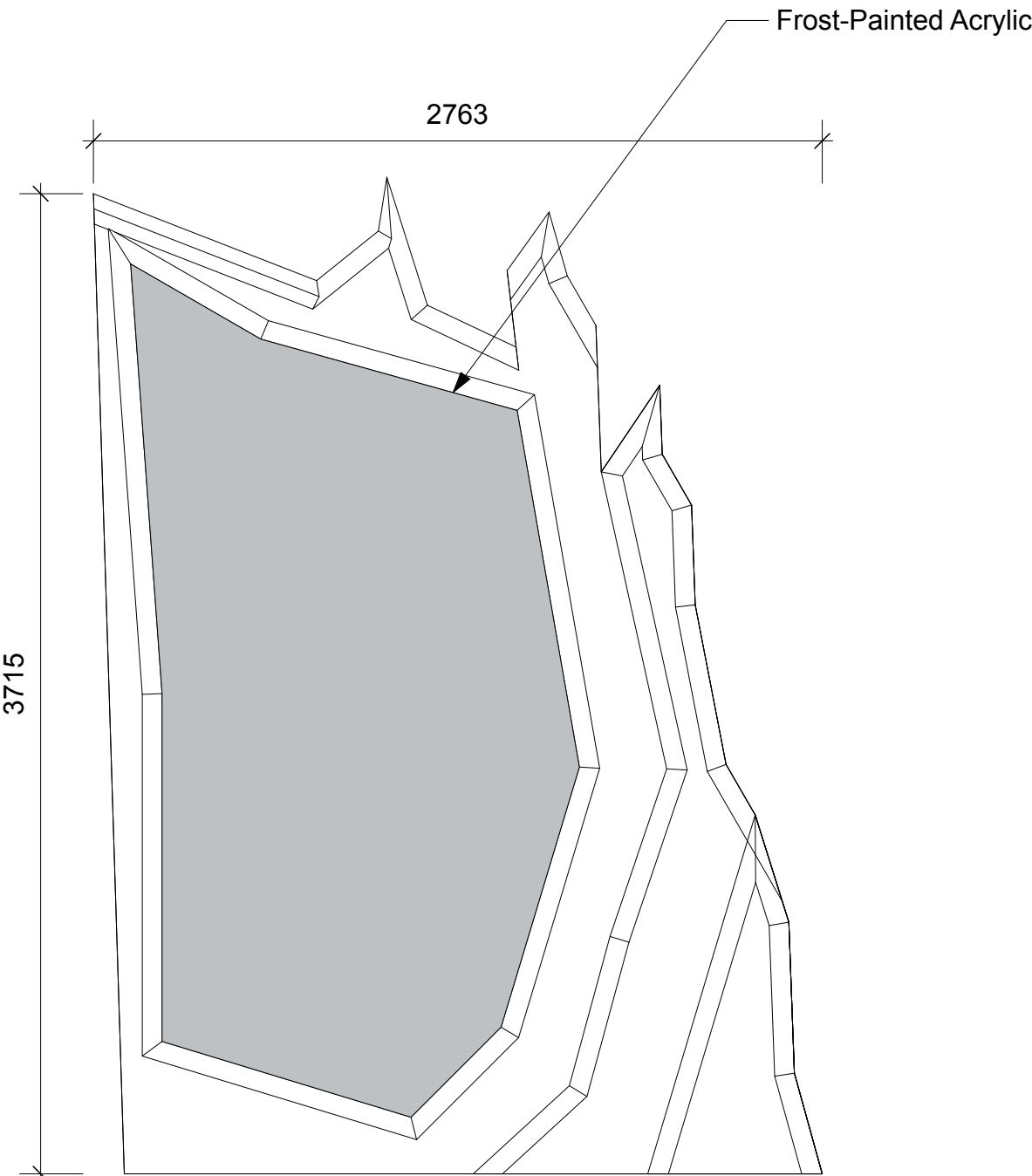
09 Ice Palace PS Front Scale 1:25
