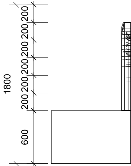
06 Staircase Piece 2 Side Scale 1:25
