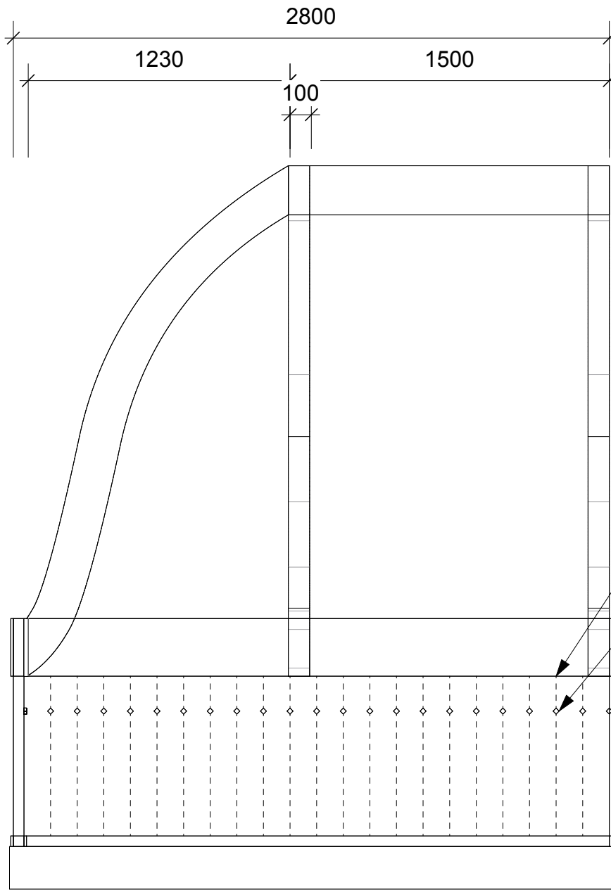
01 Bedrom Front Scale 1:25
