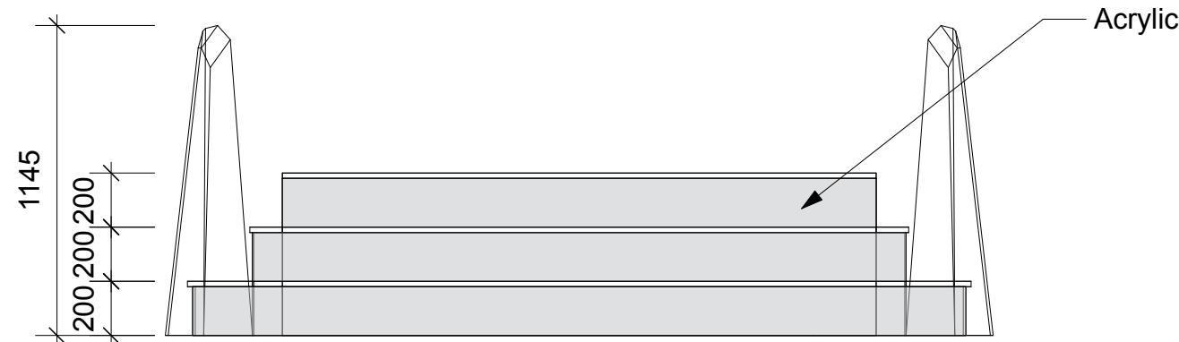
02 Staircase Piece 1 Front Scale 1:25
