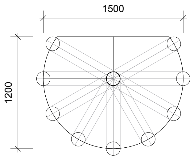
02 Bonfire Top Scale 1:25
