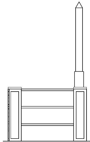
03 Chapel Stage Side Scale 1:25
