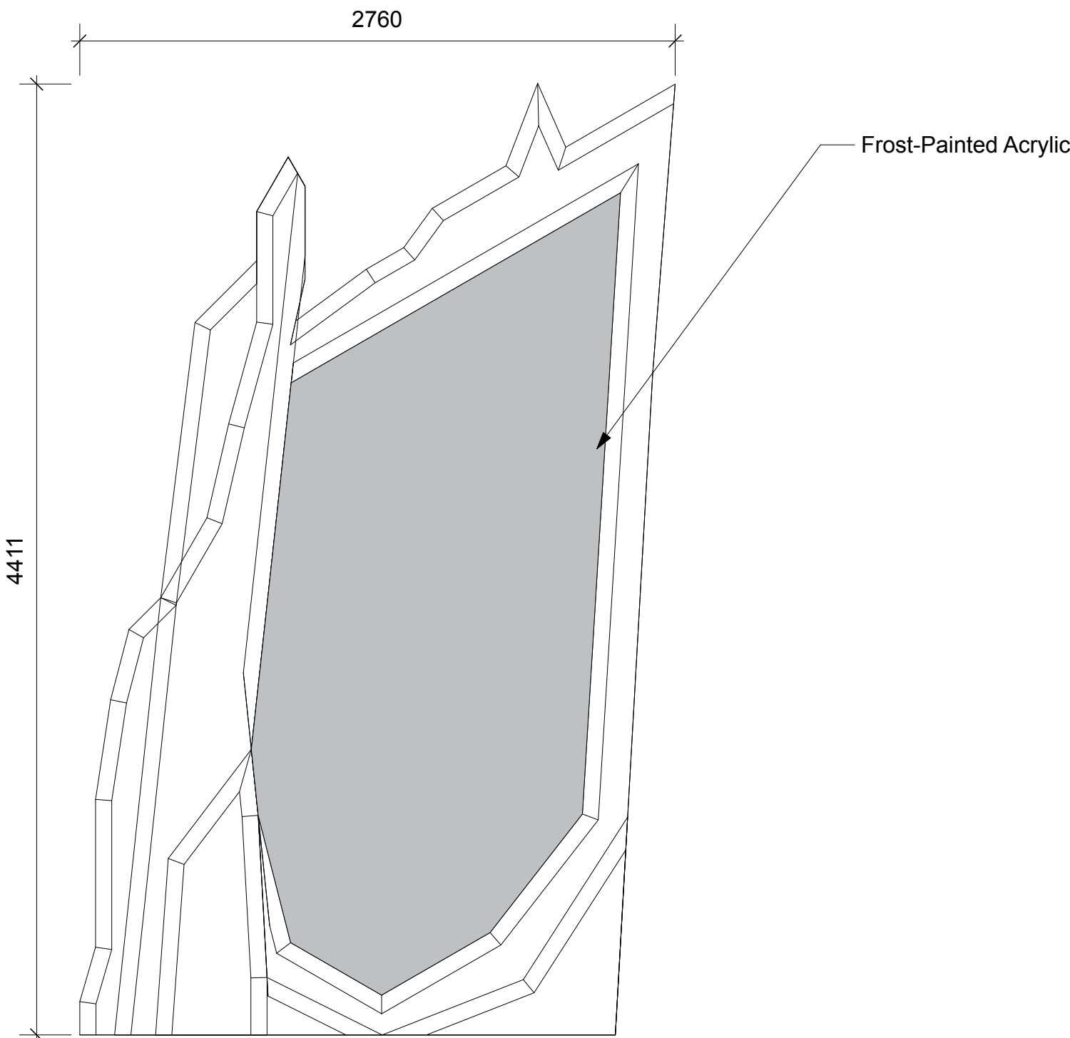
04 Ice Palace OP Front Scale 1:25
